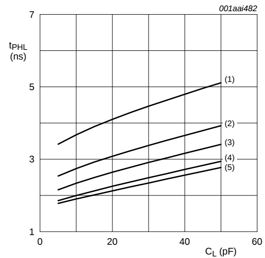
b. HIGH to LOW propagation delay (An to Bn); V_{CC(A)} = 1.8 V
